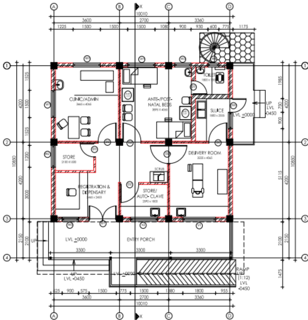
GROUND FLOOR PLAN Area: 107.57 Sq. M.
